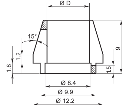
Collets for 8.0 mm
