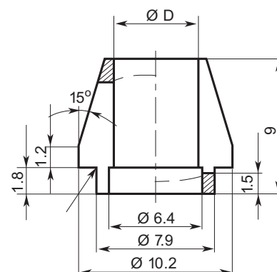
Collets for 6.6 mm
